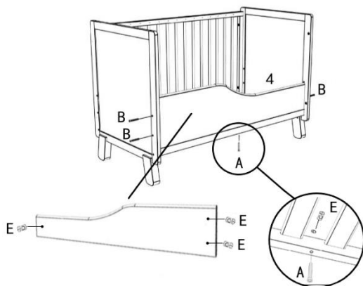
IIIa
