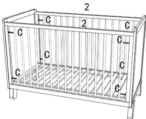
IIIa
